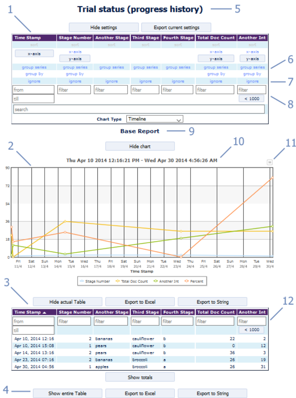
Figure 2: A complete overview of Fusion Interface in myInsight
