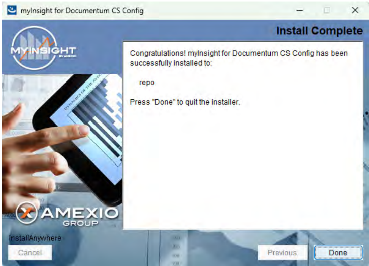
Figure 23: Installation completed
