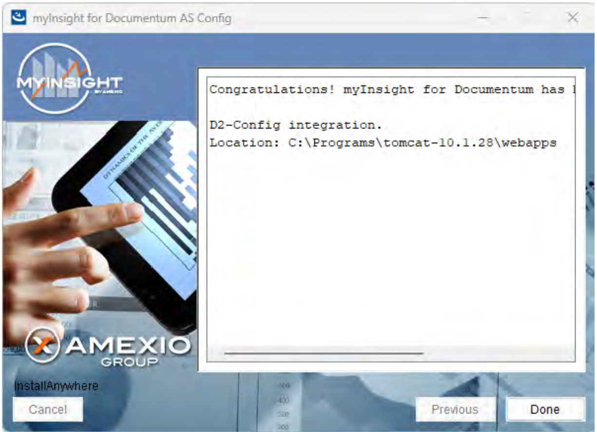
Figure 49: Installation completed
