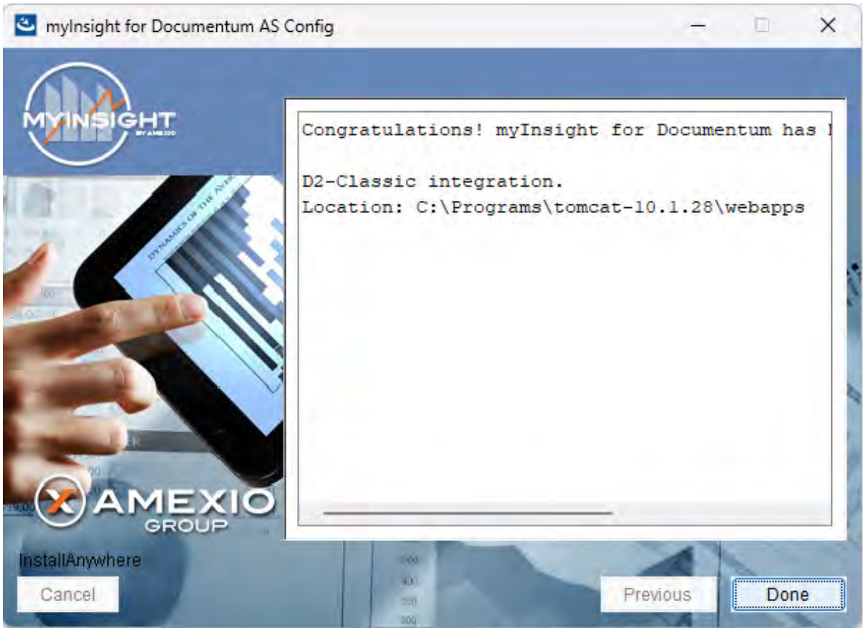
Figure 61: Installation completed
