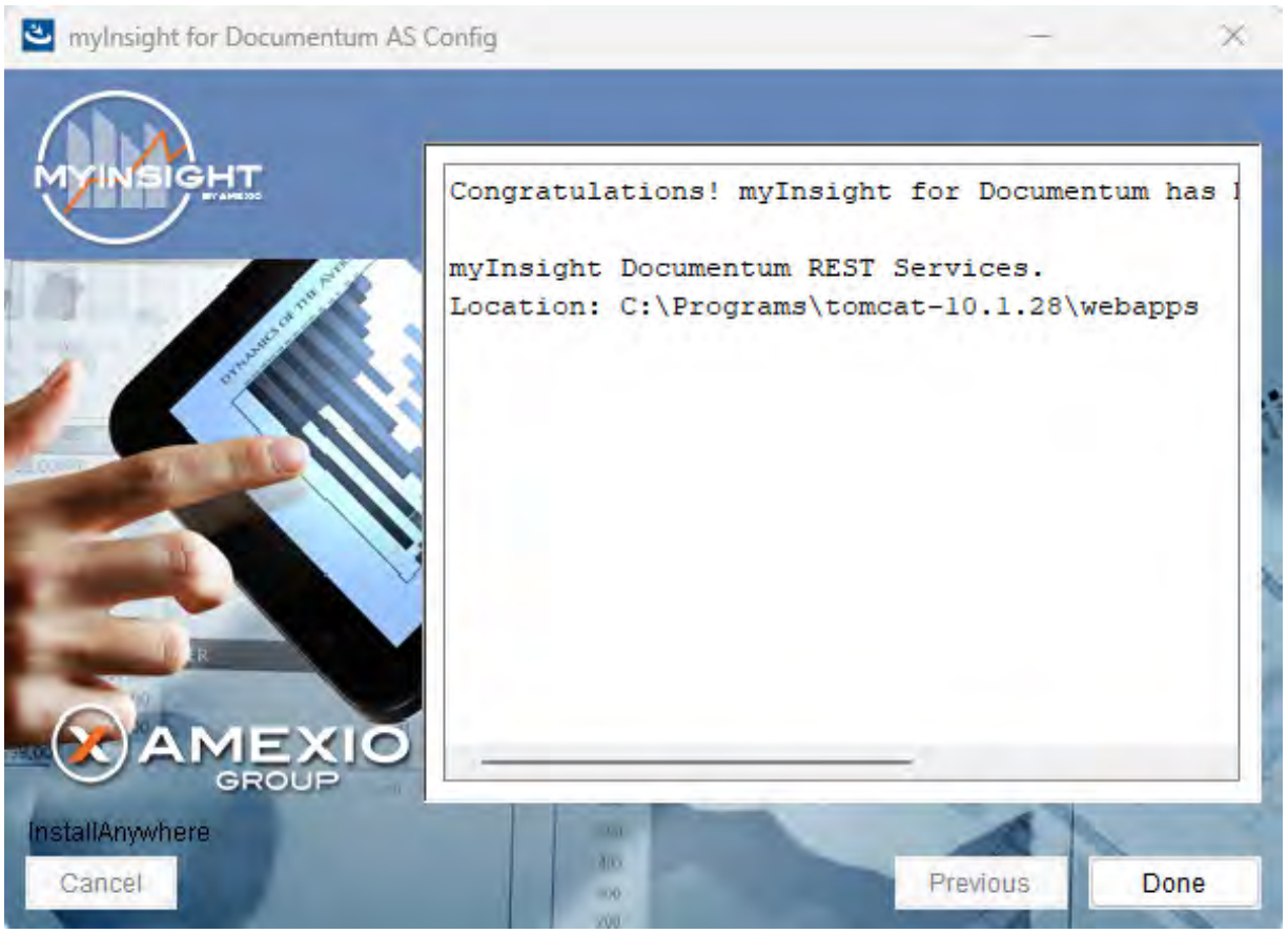
Figure 72: Installation completed
