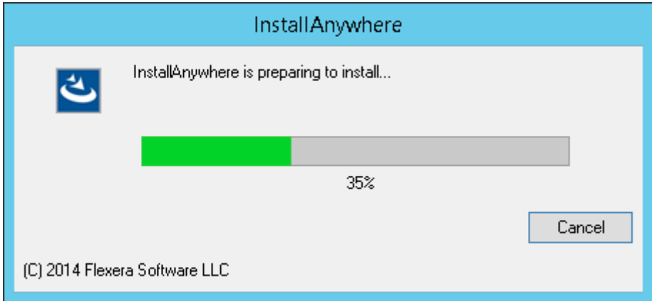
Figure 27: Initializing installer
