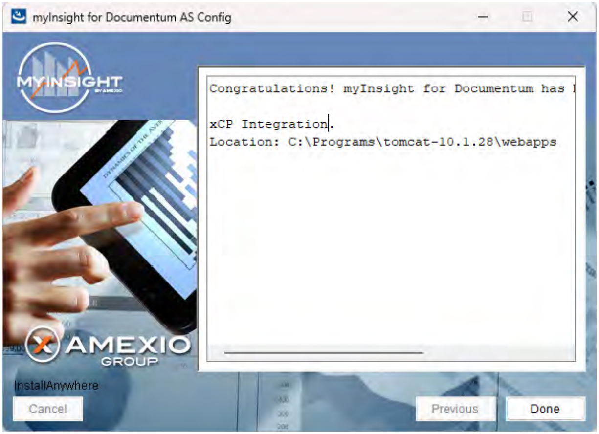
Figure 96: Installation completed
