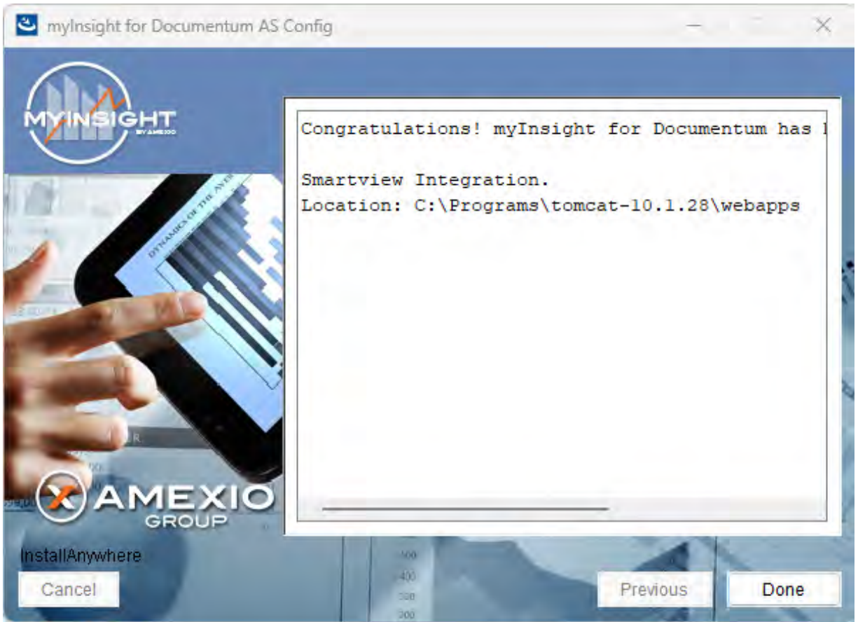
Figure 38: Installation completed
