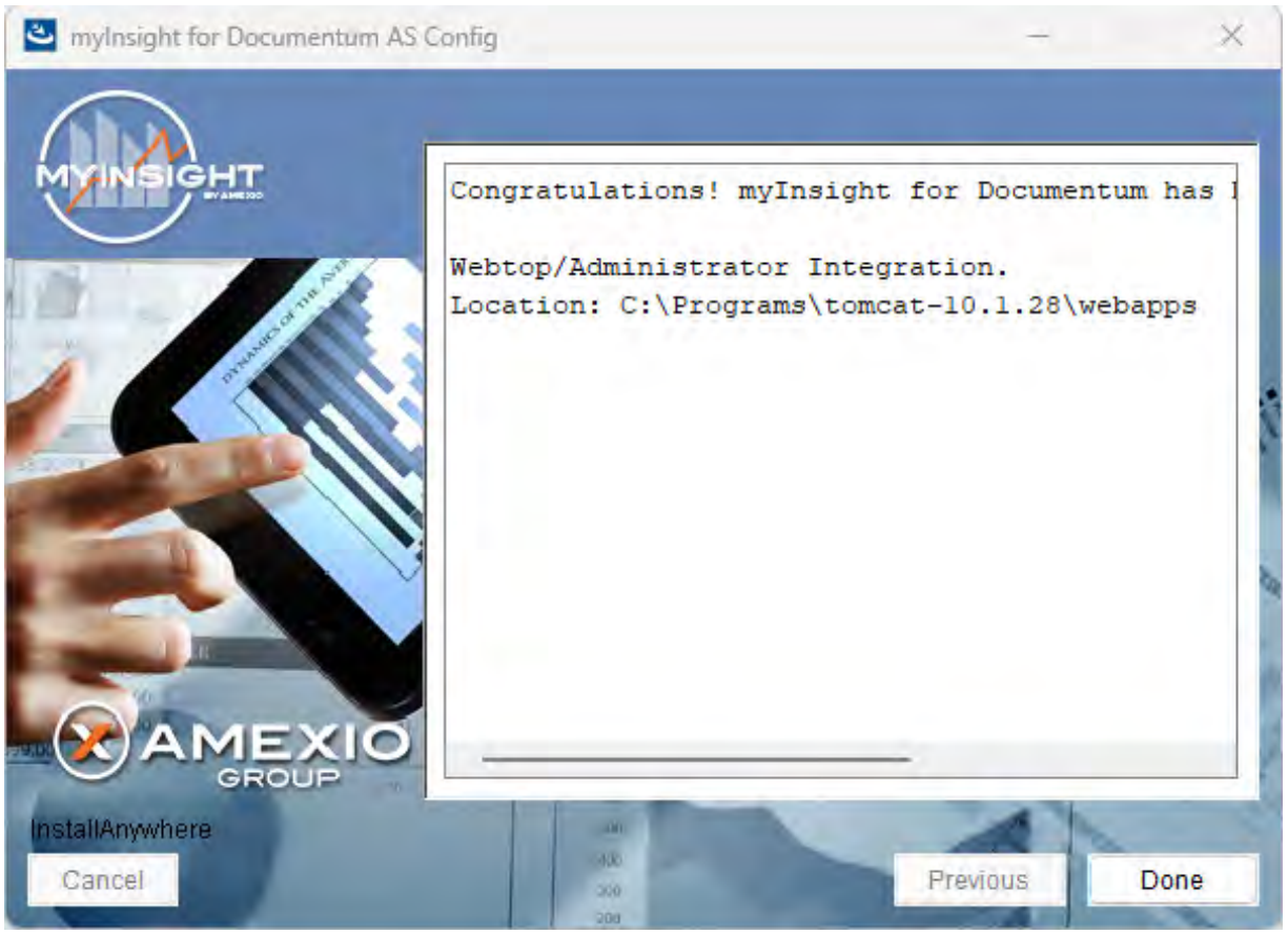
Figure 84: Installation completed
